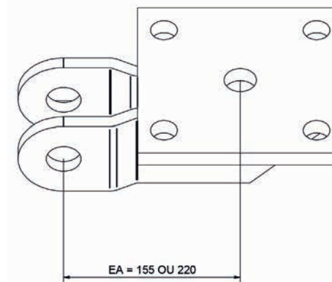
PLAQUE SUPPORT BIELLE
